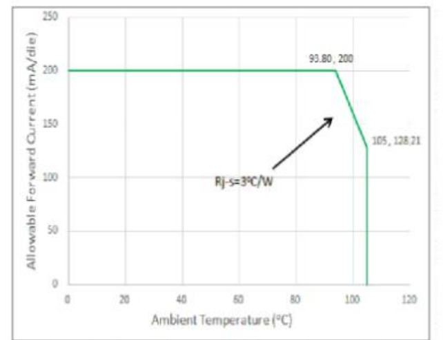
Fig 10 .Maximum Forward Current vs. Ambient Temperature
