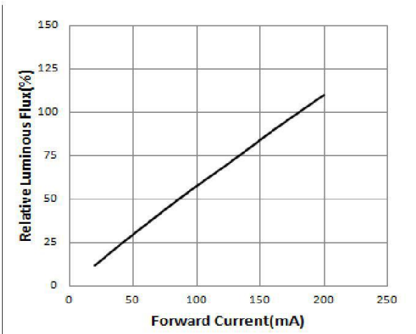
Fig 5. IF vs. Relative Luminous flux
